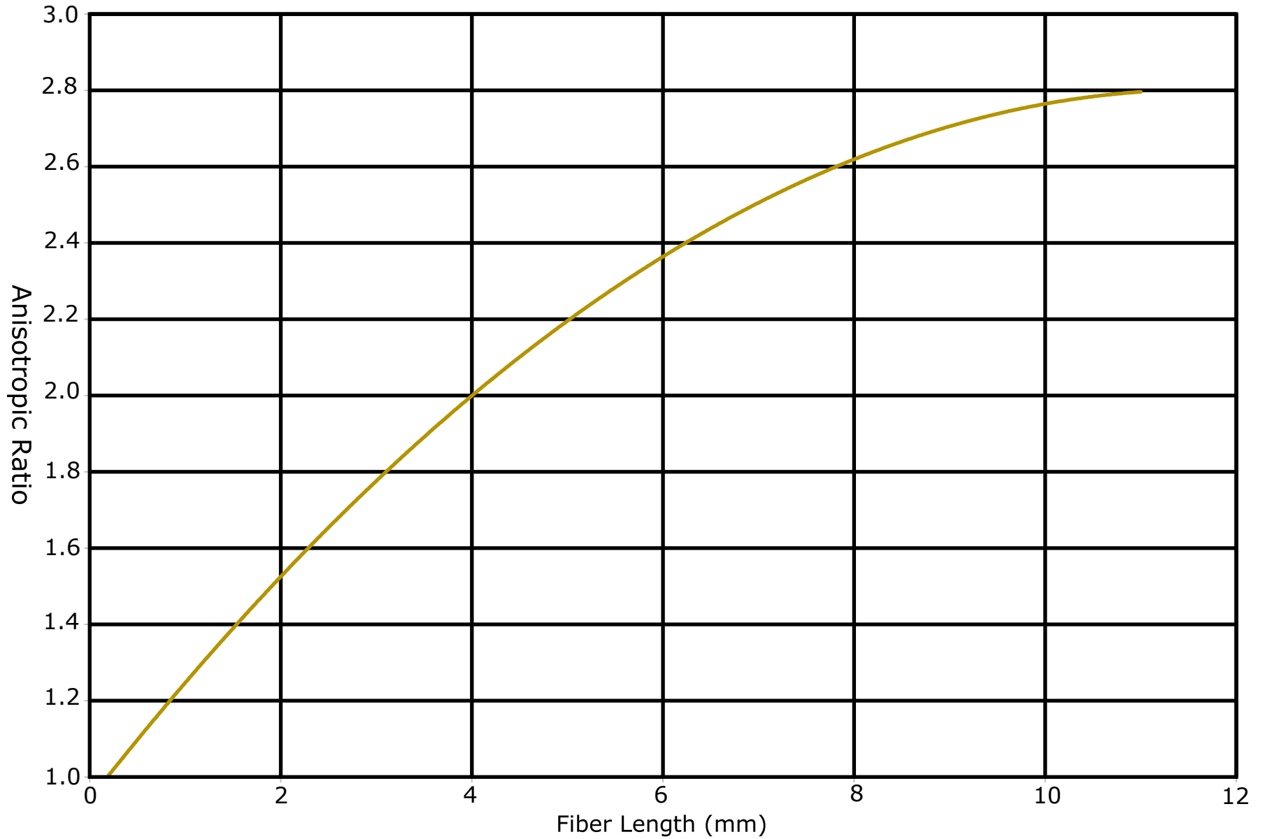
Anisotropic Ratio: (with grain mod)/(cross grain mod)
